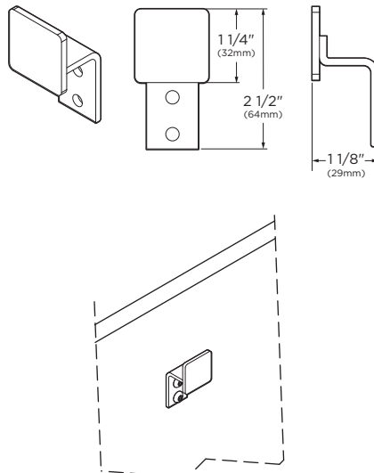
#1000869 Coat Hook
