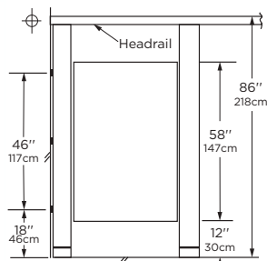
1542 Series Overhead-Braced
