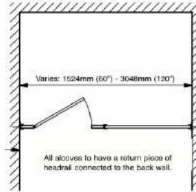
alcove plan
