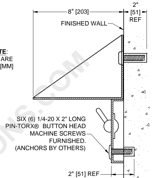
A-SECTION VIEW
