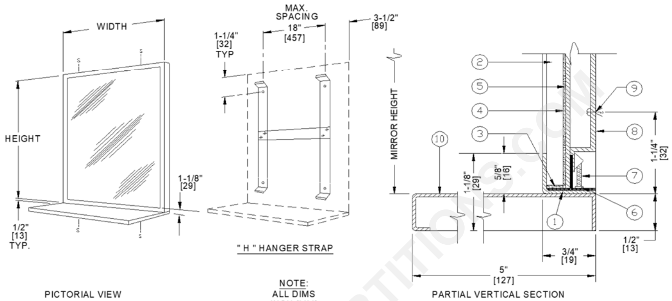
PICTORIAL VIEW
