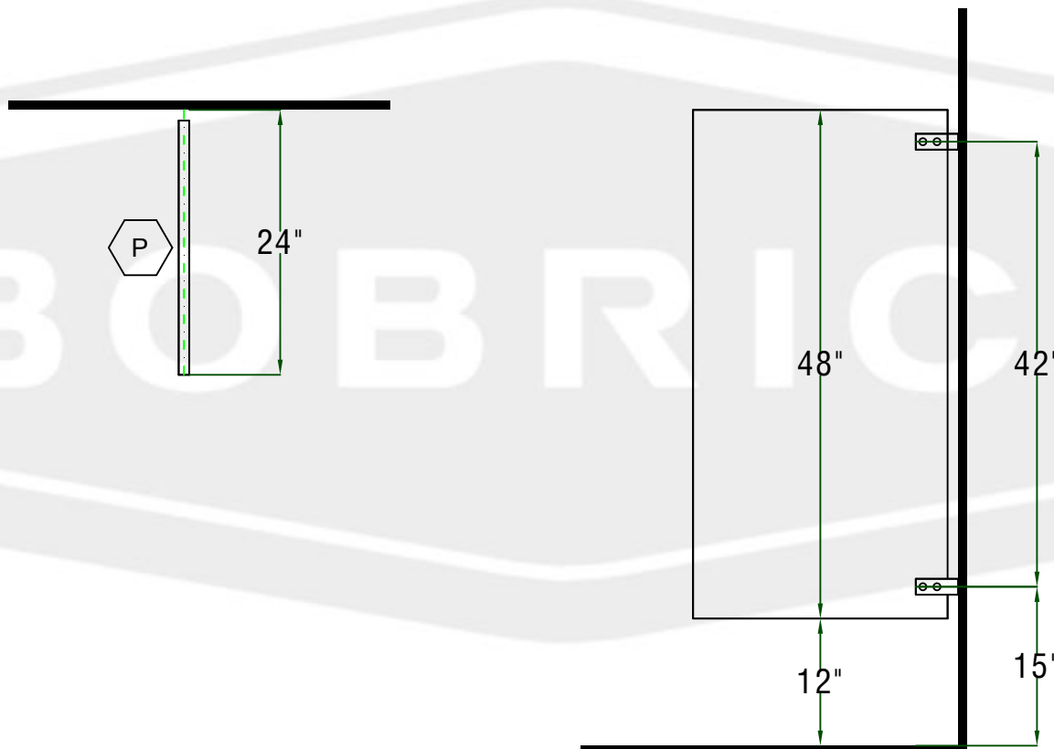
PLAN VIEW
