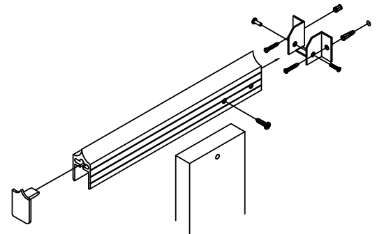
Headrail Brace
