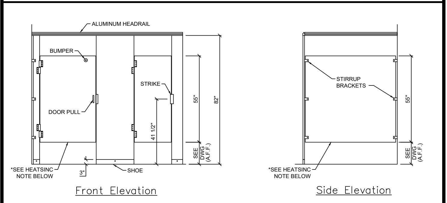
Plan Elevation
