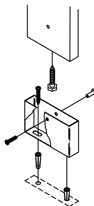
Floor Mount
