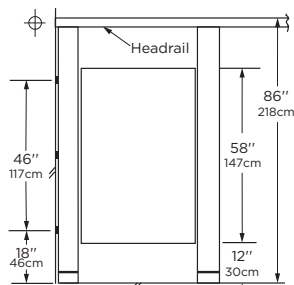
1542 Series Overhead-Braced
